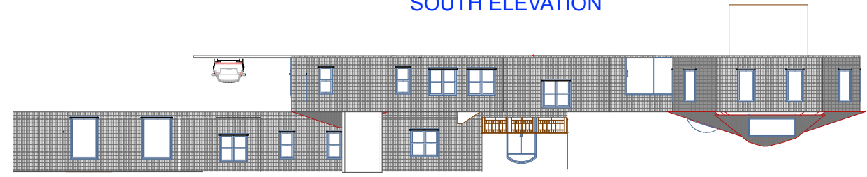
SOUTH ELEVATION
