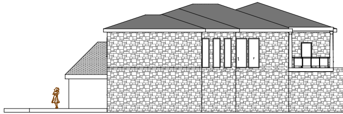
SOUTH ELEVATION
