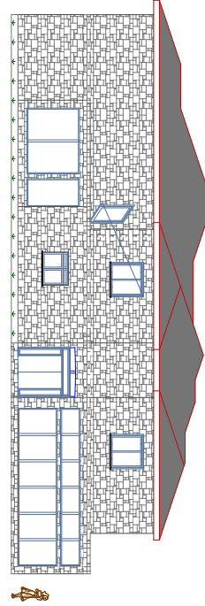
WEST ELEVATION
