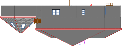
SOUTH ELEVATION
